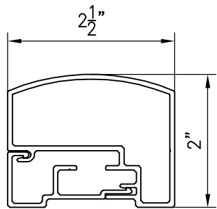
Bottom Rail RB-100/101
