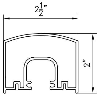
Top Rail RTNG-102
