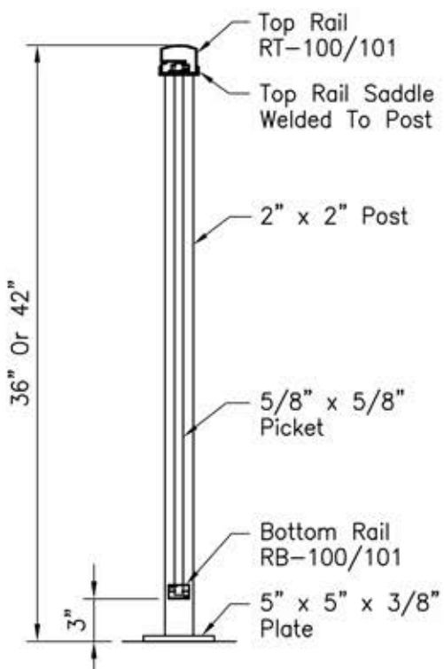
Picket Sections
