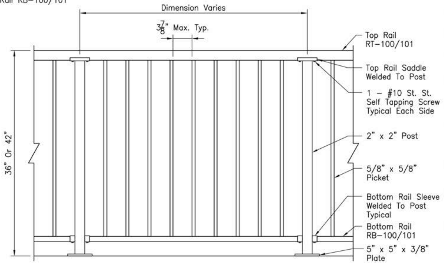
Picket Elevations
