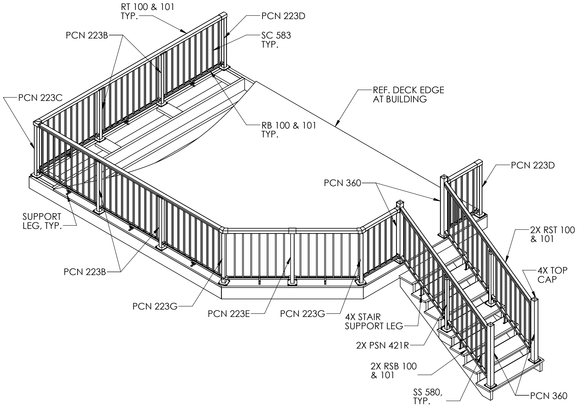
S.T.A.R. - PICKET DECK - GENERAL VIEW
