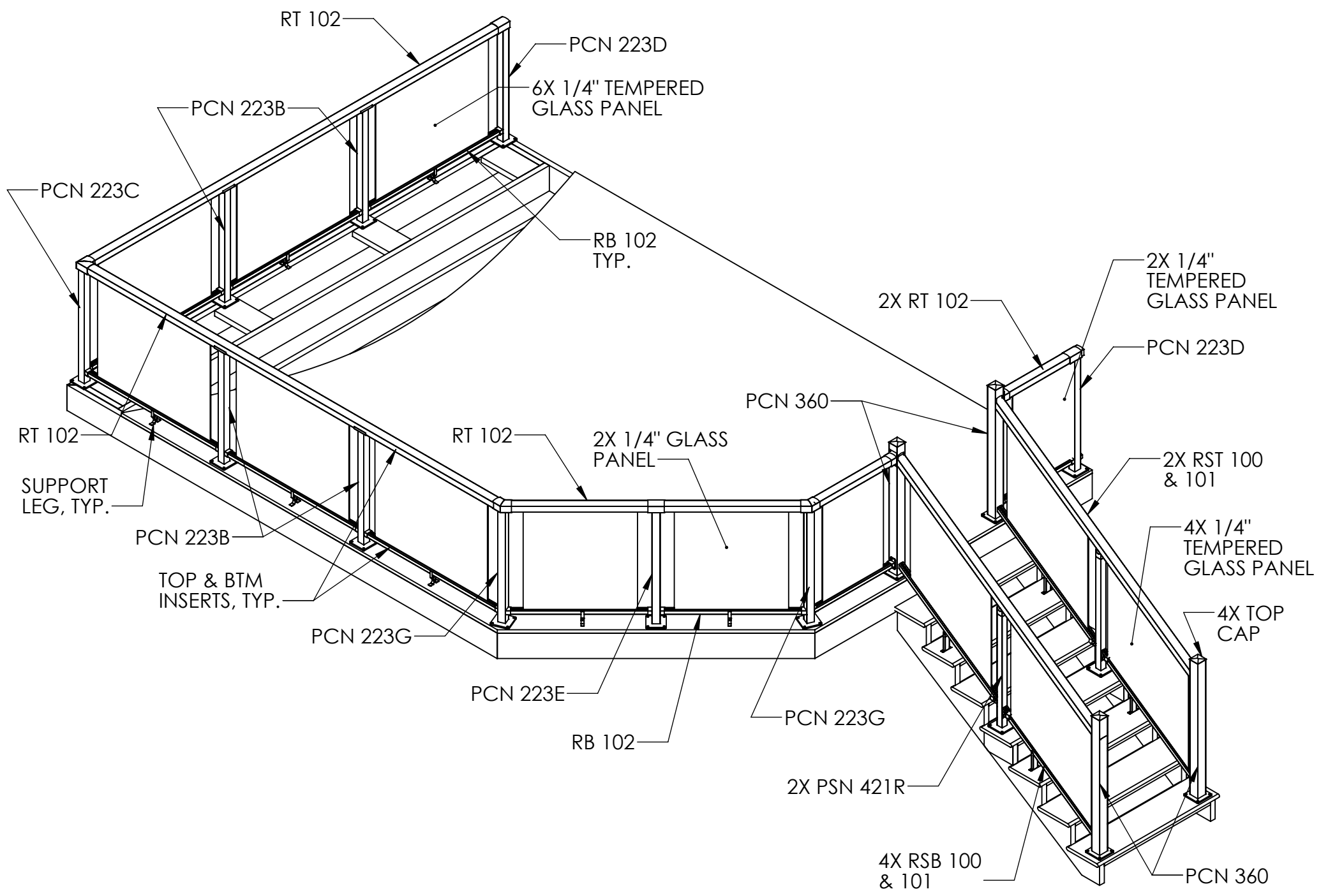
S.T.A.R. - GLASS DECK - GENERAL VIEW
